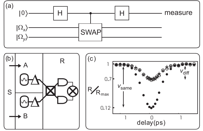
FIG. 1. (a) Quantum circuit of the original fingerprinting protocol [2,3]. (b) Linear optical implementation: Alice (A) and Bob (B) each receive a two-bit message from Sapna (S) and a single photon in a known polarization state from a source. The photons are transformed (represented by \Delta ) to particular tetrahedral states according to the received message. The photons are sent to Roger (R) who mixes them at a symmetric beam splitter \boxtimes and uses coincidence detection (two detectors \square and a multiplier \otimes ) to infer if the messages were the same or different. (c) Coincidence dip with state |\Omega_1\rangle mixed with |\Omega_0\rangle ( \circ ), |\Omega_1\rangle ( \bullet ), |\Omega_2\rangle ( + ), and |\Omega_3\rangle ( \times ). The plots correspond to the normalized coincidence rate R/R_{\text{max}} (with R_{\text{max}} = 474 \text{ s}^{-1} the maximum observed rate, or background rate, for the HOM dip) vs the relative delay between two photons. v_{\text{same}} and v_{\text{diff}} represent the dip depth 1 - R_{\text{min}}/R_{\text{max}} for photons in same or different states, respectively.
